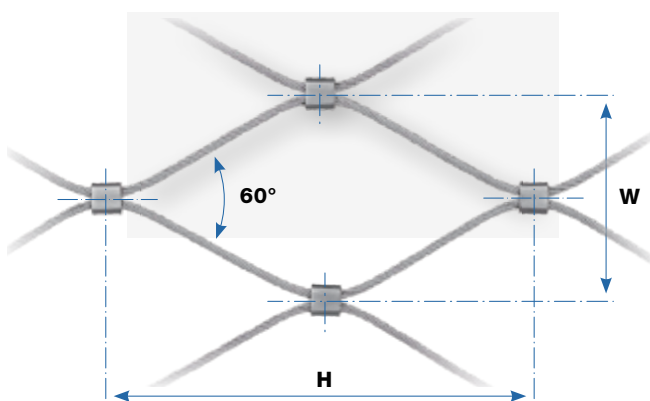
Webnet micro mesh standard
